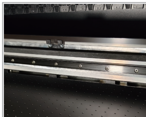
Industrial Belt Drive + Plastic Diffraction Grating
